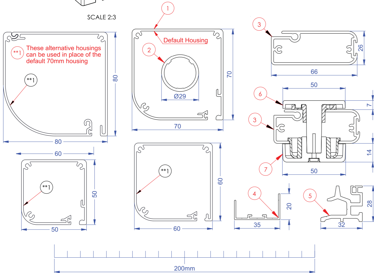
Freedom Screens Zipline COMPONENT DIMS - GENERAL Scale 1:1 at a3 Revision-006
